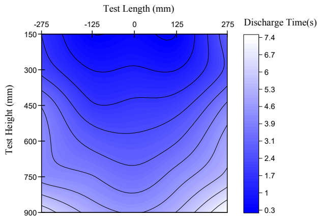
Discharge time distribution diagram of AP-DJ2812
